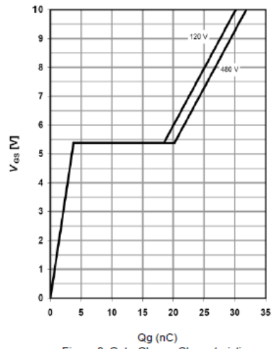
Figure 8: Gate-Charge Characteristics
