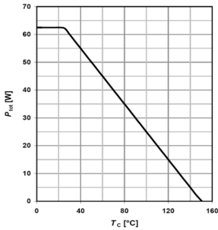
Figure 3: Power Dissipation
