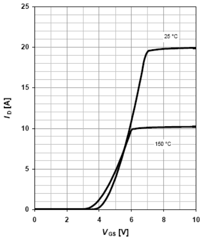
Figure 13: Typ. transfer characteristics
