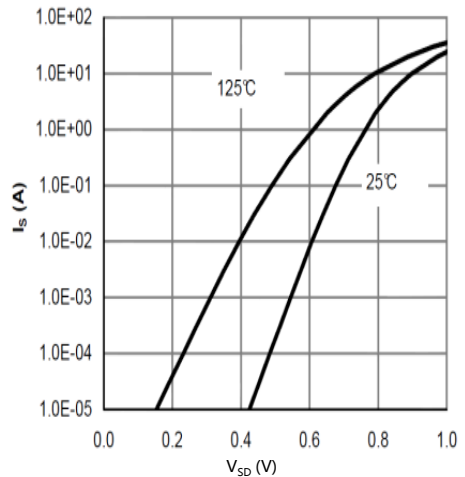
Figure 6: Body-Diode Characteristics
