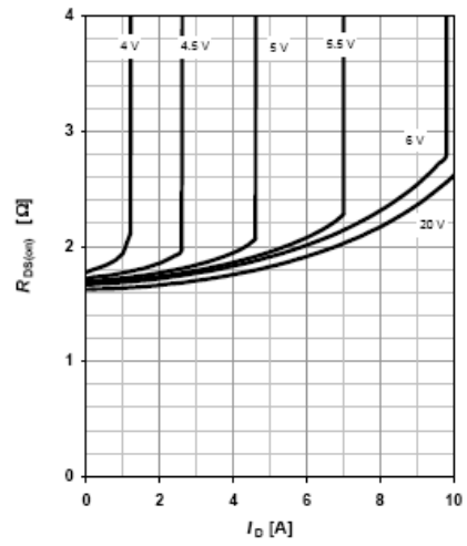
Figure 14 On-Resistance vs. Drain Current
