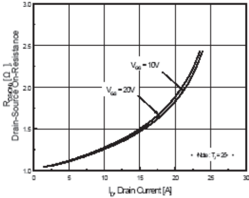
Figure 3. On-Resistance Variation
