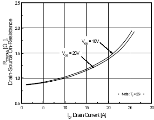
Figure 3. On-Resistance Variation
